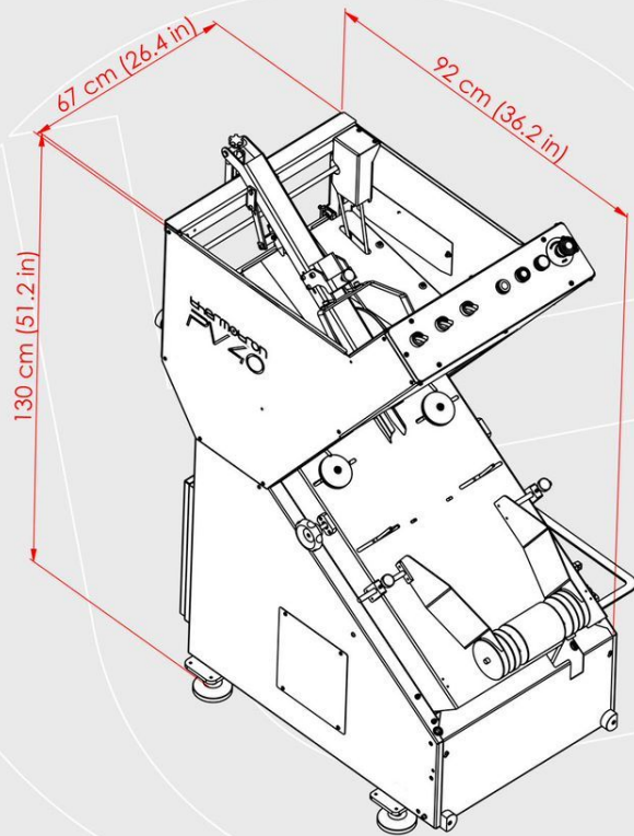
PV40 [ISOMETRIC VIEW]
